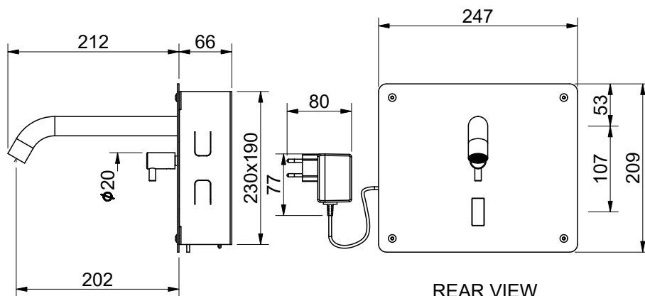
REAR VIEW
